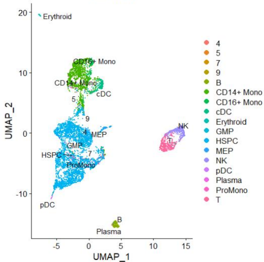
scAnnoX
