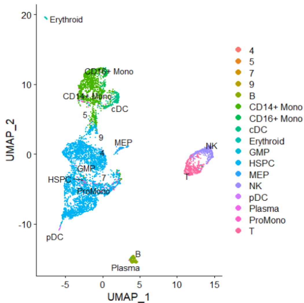
scAnnoX
