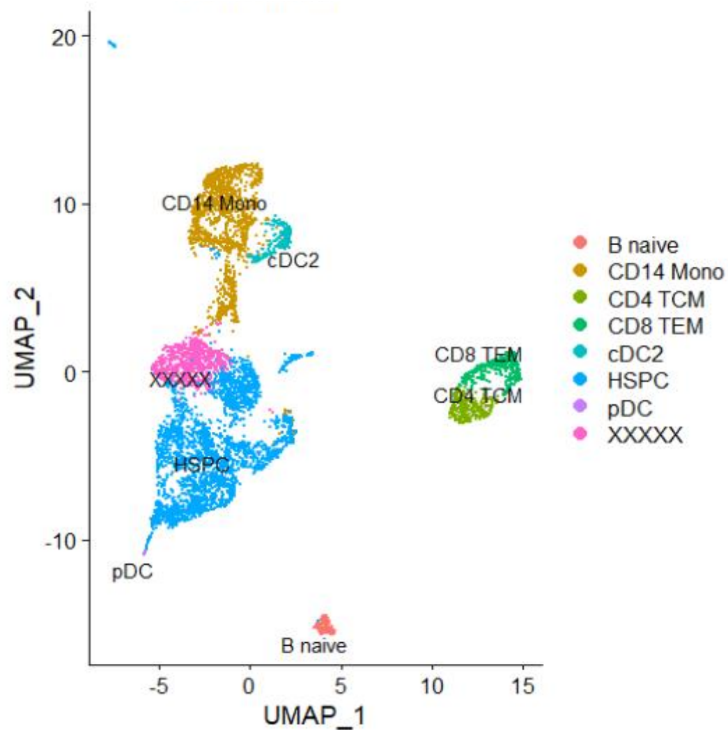
Annotated data
