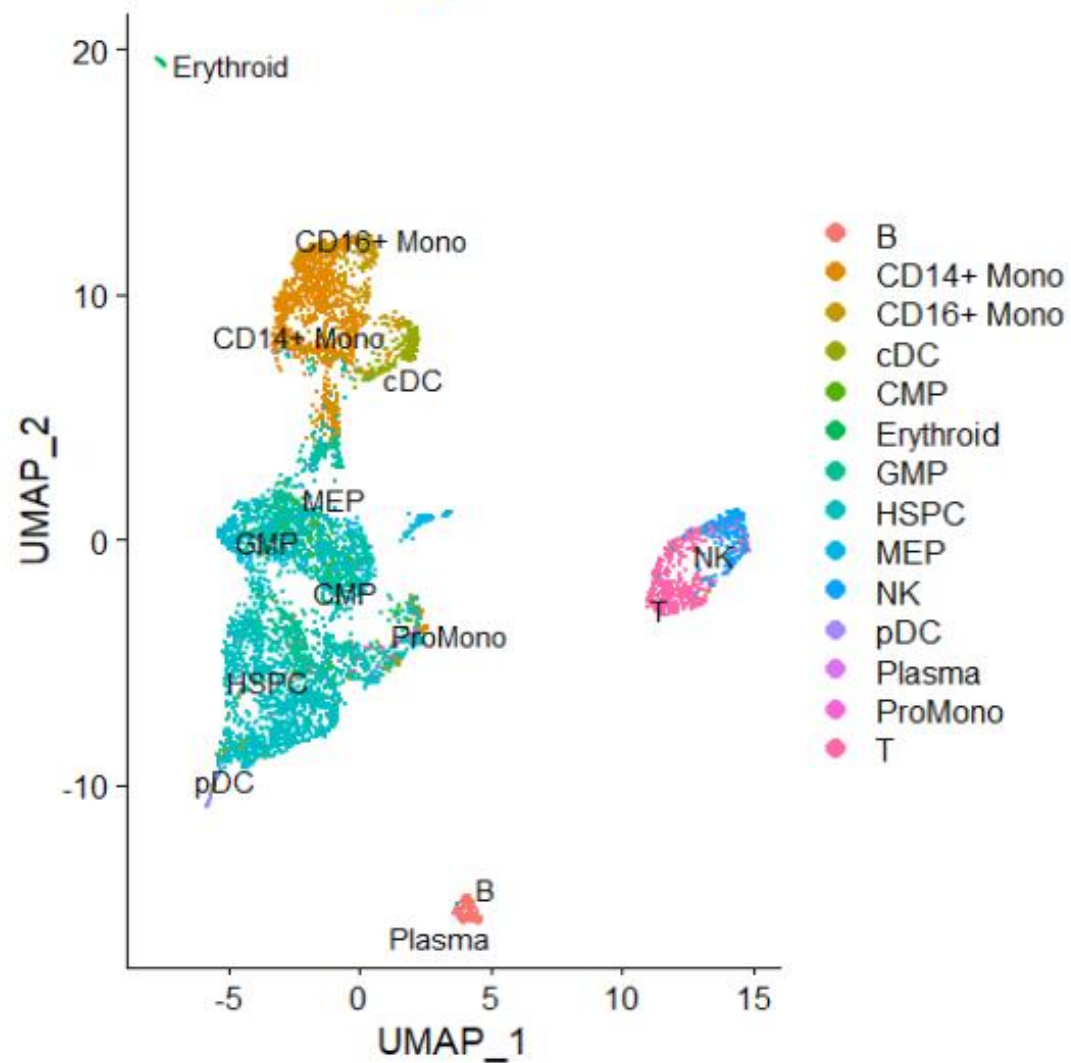
singleR
