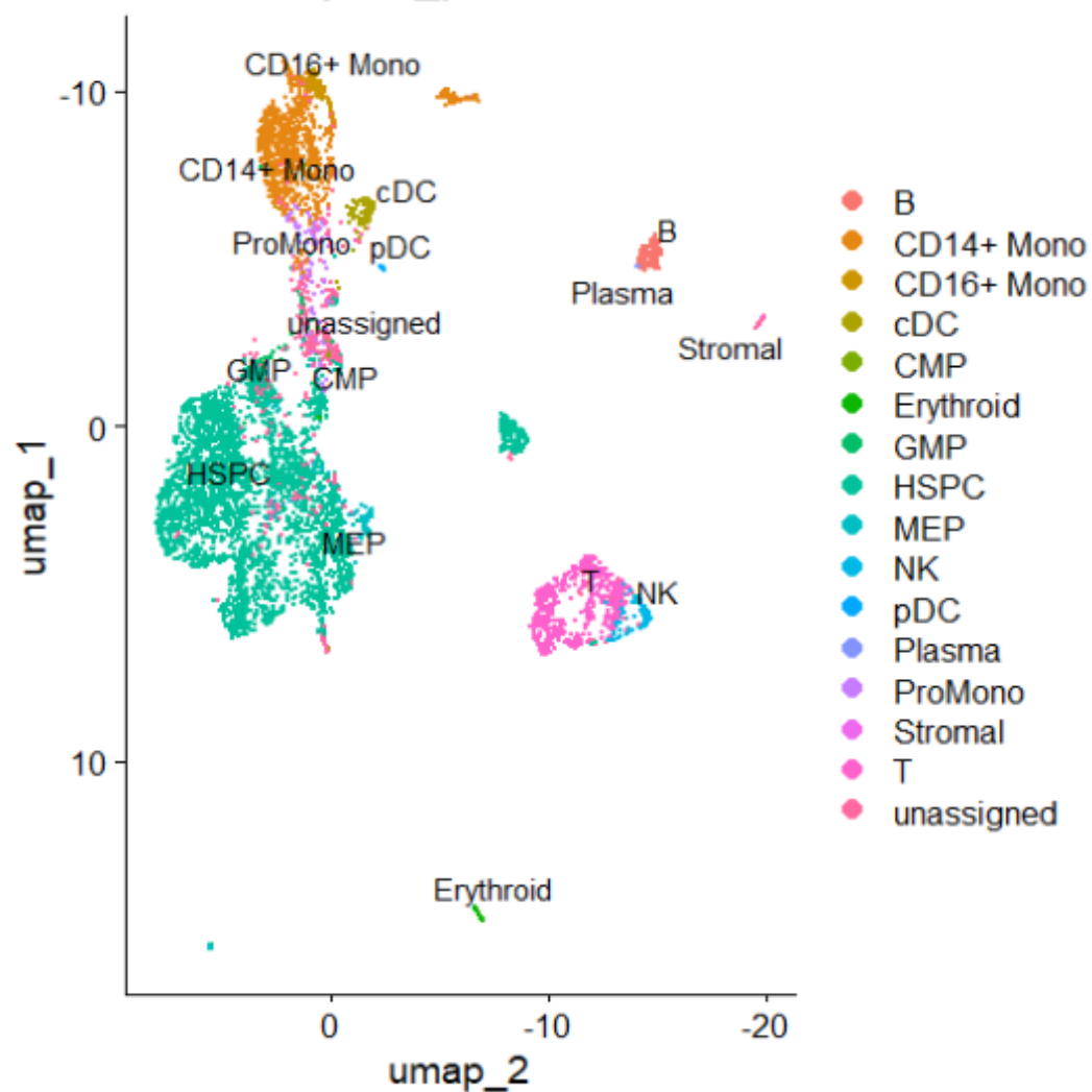
scpred_prediction
