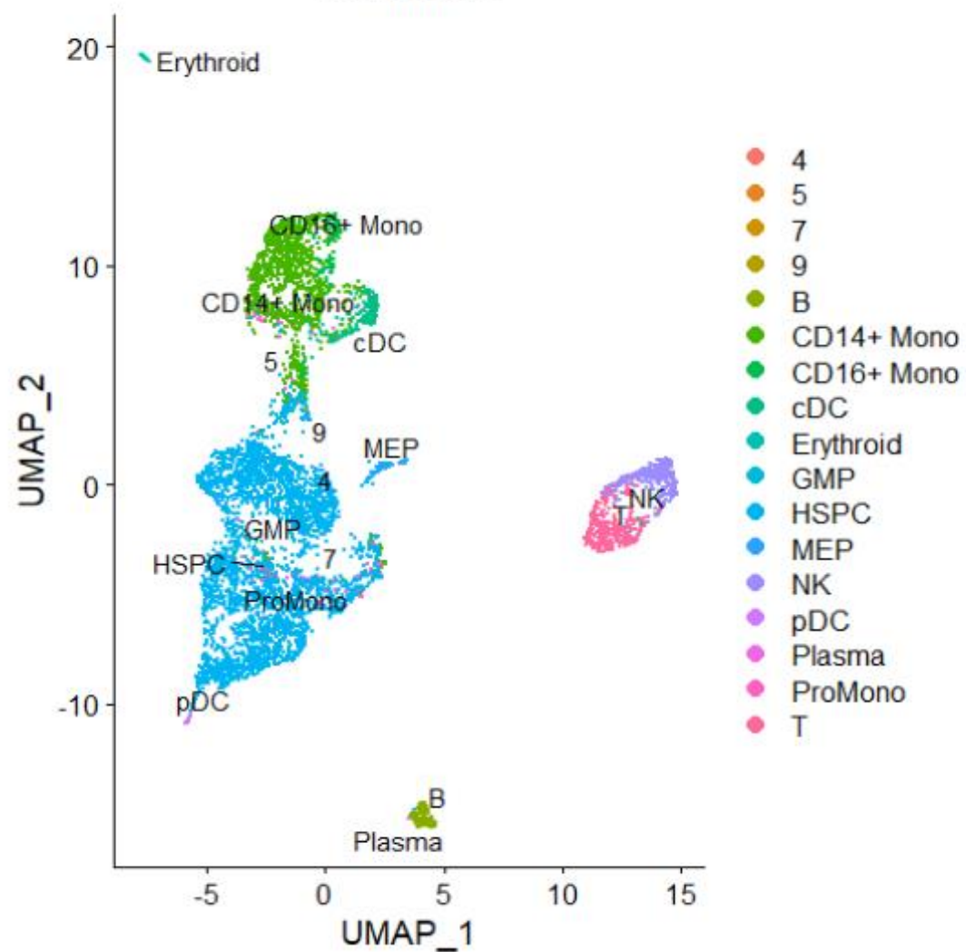
scAnnoX
